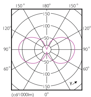
LED Bulb CLA 8-50W E27 G120 Amber 822 DIM
